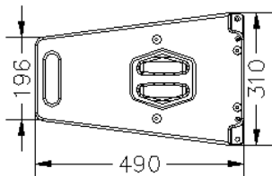
边视图/Side
