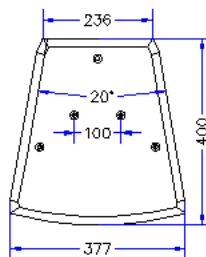
顶视图/Top
