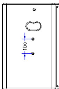
边视图/Side
