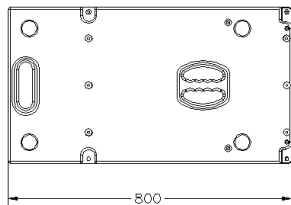
边视图/Side
